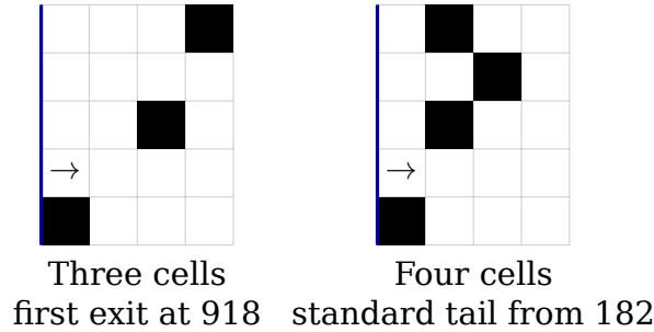
Figure 1: The sharp three-cell witness B_* and the four-cell port G . Cell coordinates refer to square centres. The ant starts at (0, 0) facing east; the blue line separates columns -1 and 0 .
